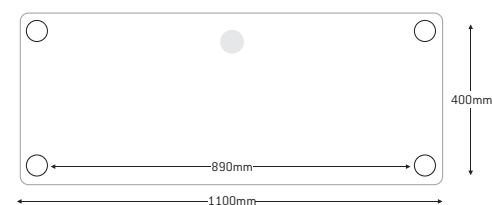
PLAN ELEVATION
